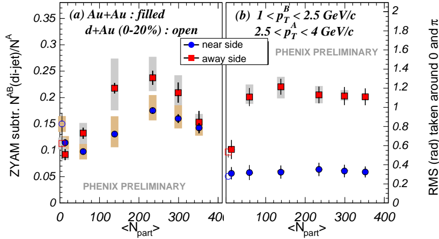
Fig. 5. (a) Associated yields for near- and away-side peaks in the jet-induced pair distribution; and (b) Widths (RMS) of the peaks. The open symbols denote results for 0-20% most central d+Au events from a recent PHENIX analysis.
